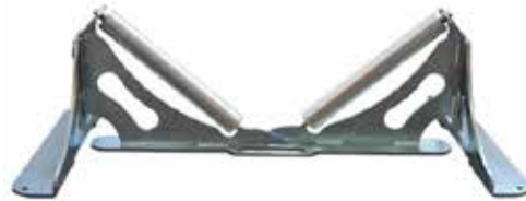
RITMO ROLLER 1000 • Supports pipes 10" - 36" DIPS
