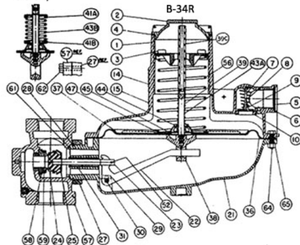
B34R Reference Schematic
