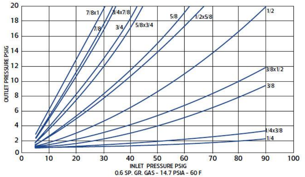
B34R Relief Curves, Blocked Open, 14" Set Point
