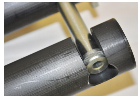
End nut inside bottom bar pocket
